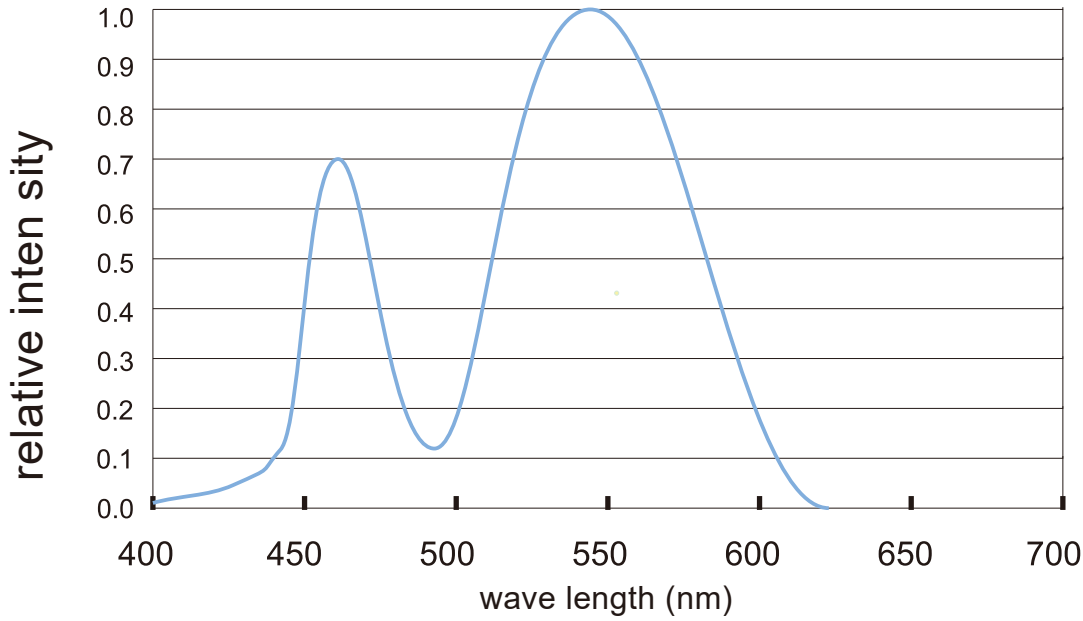
Radiation diagram
