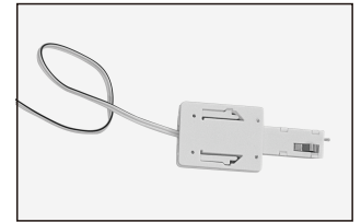
ITR001-HP (Max 2A) Cable length 35mm.
