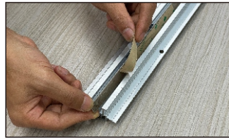
Insert two tracks (Code: STR02-HT) into the groove on both sides of STR002.
