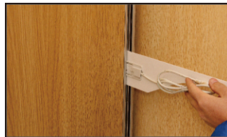
Insert two STR002-HM into the STR002 on the left and right ends respectively.
