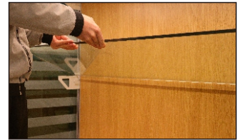
Insert the glass plates into the slot on the corresponding STR002-HG and fix it.
