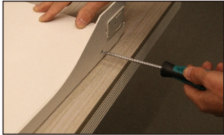
Fix the STR002-HL/HR on both sides of the wooden board with screws corresponding to the position of the expansion screw plug.
