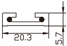
Model: TRACK01 Track: 25A max. 12VDC/24VDC
