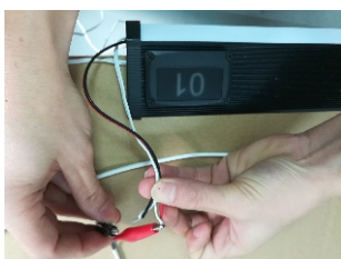
Step 9 LED light connect to power supply (black-,red +)
