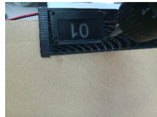
Step 6 fixed the row number by M3*16 screw on the profile
