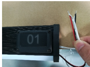
Step 7 led strip + connect to row number +, led strip- connect to row number - (black-,red +)
