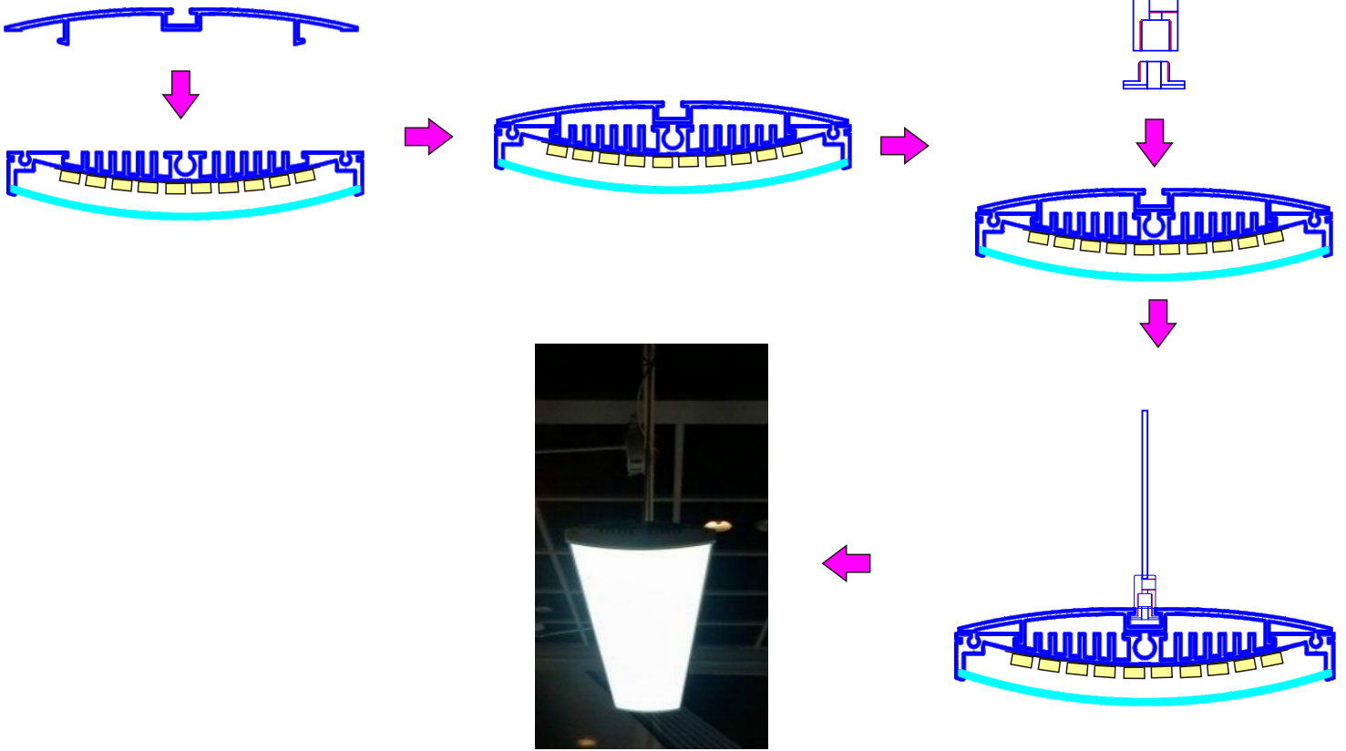
Fix the top joiner to the ceiling. Adjust the cable length to suit
